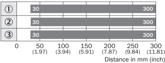
Sensing range diagram WTB8, 300 mm
