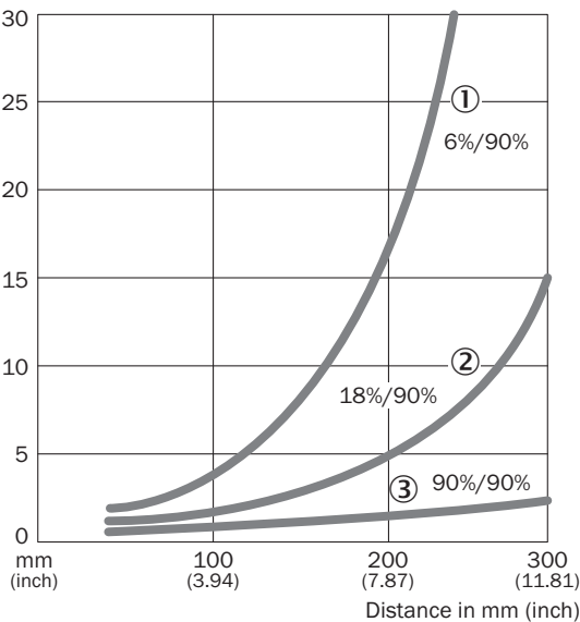
Characteristic curve WTB8, 300 mm
