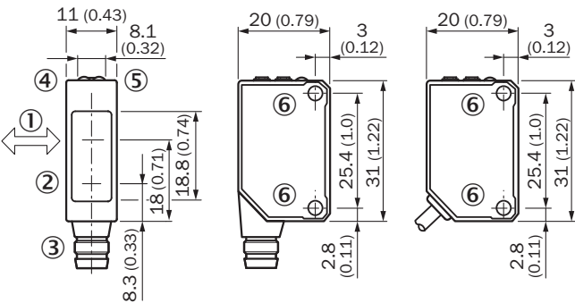
Dimensional drawing
