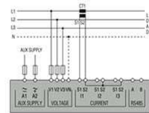
Balanced 3-phase connection with or without neutral
