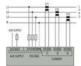
Three-phase with or without neutral
