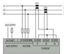
Three-phase without neutral in ARON connection
