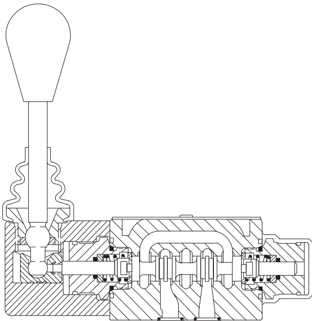
DG17V-3-* - 60 Lever Operator
