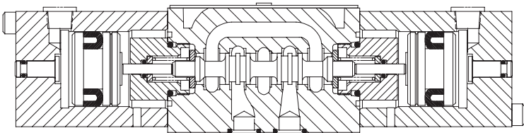
DG18V-3-* -60 Air Operator
