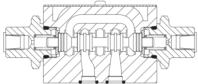
DG3V-3-* -60 Hydraulic Operator
