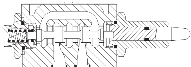
DG21V-3-* - 60 Plunger Operator
