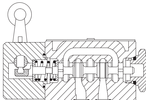
DG20V-3-* - 60 Cam Operator
