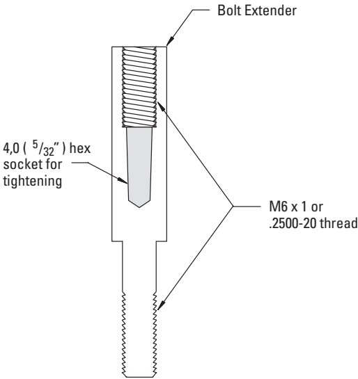
Bolt extender cross section
