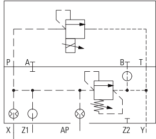
KCG-3 Proportionalventil
