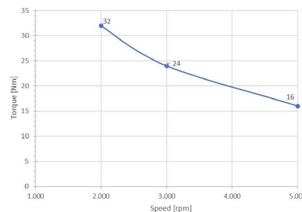
Drive torque at speed
