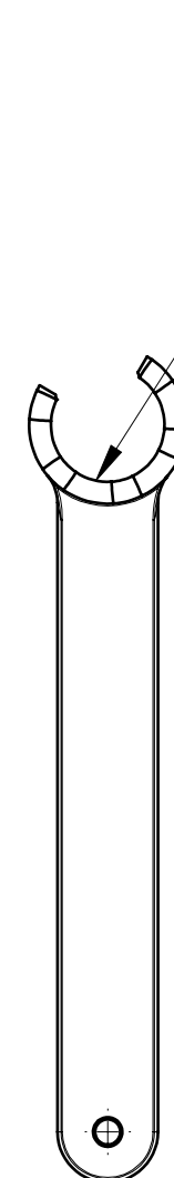
Wrench for spindle RE-44x57-ER40
