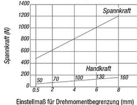
Schwenkspanner K0912....4540
