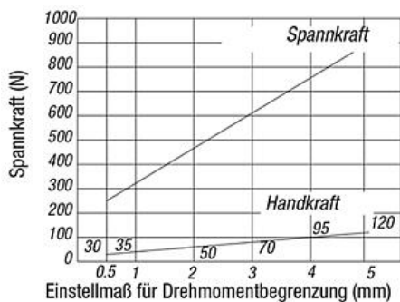
Zugspanner K0910.3240...
