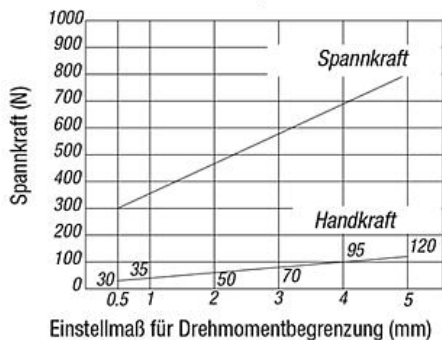
Schwenkspanner K0912....3232
